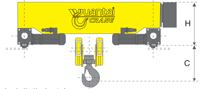
NWH双梁钢丝绳电动葫芦选型表 Selection table of NWH double girder wire rope hoist
